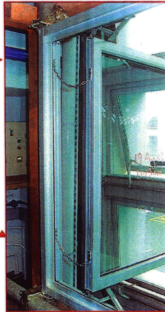
One pair of safety devices close-up view
